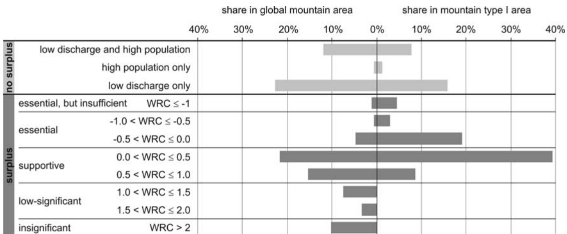
Figure 7. Importance of all mountain areas (left) and of Earth system mountain type I (right) for lowland water supply, assessed through occurrence of water resources contribution index WRC . Note that mountain type I shows no WRC values above 1 and therefore always has at least supportive function; this complies with its definition as a mountain area with high contributing potential to a dry lowland area (see also Table 2).
