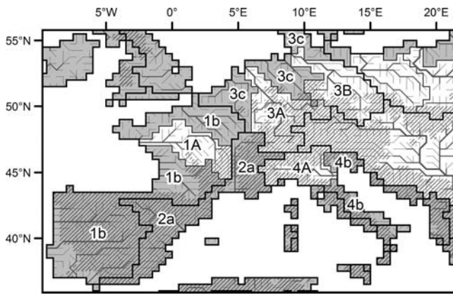
Figure 1. Hydrological division of continental surface into “analysis basins” using the simulated topological network STN–30p boundaries [Vörösmarty et al. , 2000a, 2000b] for river basins with a surface area larger than 100,000 km 2 (white) and the coastal catchments typology [Meybeck et al. , 2006] for the remaining areas (dark gray). Mountain areas are shown in hatch marks. Samples: 1A = Loire River basin (118,282 km 2 ), 1b = remaining Iberian-Biscay coastal catchment; 2a = Balearic coastal catchment (no large river basins contained); 3A = Rhine River basin (165,059 km 2 ), 3B = Elbe River basin (148,530 km 2 ), 3c = remaining North Sea coastal catchment; 4A = Po River basin (102,183 km 2 ), 4b = remaining Adriatic coastal catchment. For the Po River basin the area is clearly too high since the STN–30p grid is not able to separate it from the adjoining Adige River basin [see Syvitski et al. , 2005].
