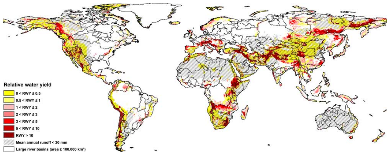
Figure 4. Disproportionality of mountain runoff formation relative to average lowland runoff ( RWY ), mapped cell by cell for mountainous areas. Disproportionality in favor of runoff is given when RWY is greater than 1, its importance being marked for RWY > 2 and essential for RWY > 5 .
