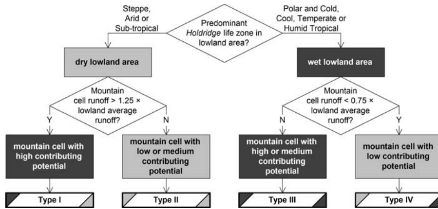
Figure 2. Flow chart for distinction of different Earth system mountain types for individual mountain cells.
