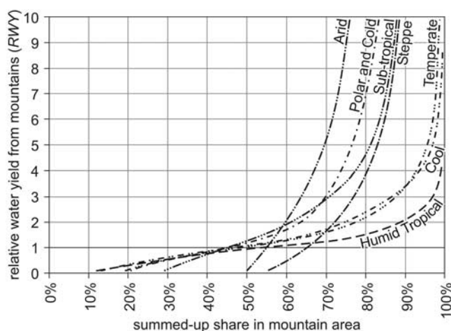
Figure 3. Relative water yield RWY in relation to the summed up share in mountain area, distinguished for seven condensed Holdridge [1967] life zones. The summed-up share refers to area-weighted cumulative distribution of RWY values; life zone distinction was made on the basis of the predominant zone occurring in the lowland area to which the mountain cell is related.
