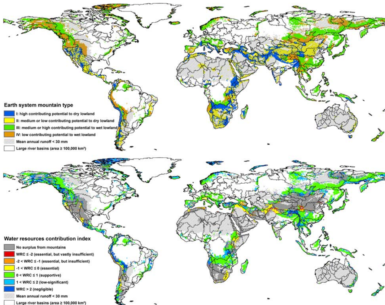
Figure 5. Global map of Earth system mountain types (top, cf. Figure 2) and of water resources contribution index WRC (bottom, cf. Table 2). Areas with an annual runoff of less than 30 mm are subject to increasing uncertainty and therefore displayed in hatch marks.
