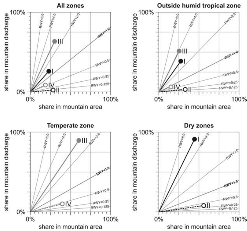
Figure 6. Share in mountain discharge (ordinate) compared to share in mountain area (abscissa), distinguished by predominant Holdridge [1967] life zone in the lowlands and by Earth system mountain types I to IV (cf. section 3.2). The diagrams thus refer to a mountain area contributing to the respective lowland life zone. Zone-specific relation to RWY is given for each diagram, determined from respective values of area and average runoff in the lowland and in the mountain section; the steeper the line for the mountain types, the greater RWY and therefore the importance in terms of runoff formation (cf. Figure 3). The thought line of unity where share in runoff is equal to share in area refers to an average RWY of 1.3 for all zones, 1.9 outside the humid tropics, 1.7 for the temperate zone, and 2.5 for dry zones. In compliance with our definition, Earth system mountain types I and II do not contribute to the temperate zone, and types III and IV do not contribute to the dry zones.
